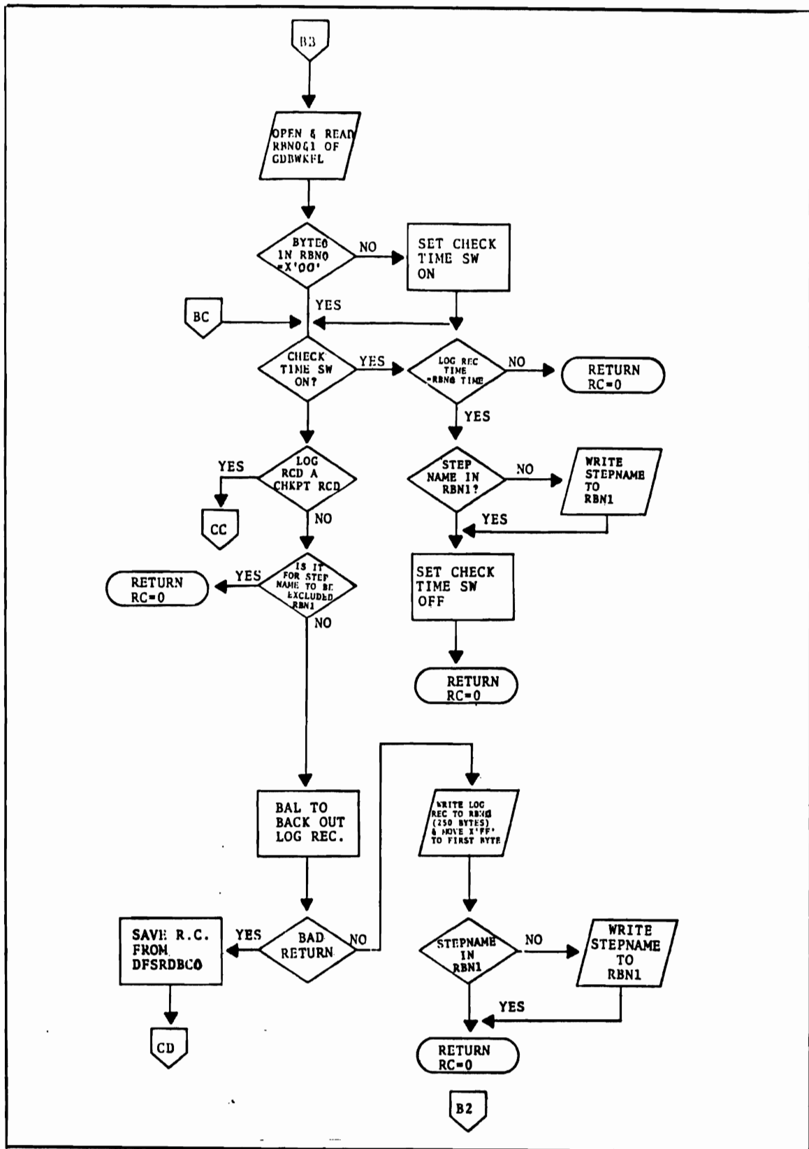
Figure 5-9. Data Base Backout Process
