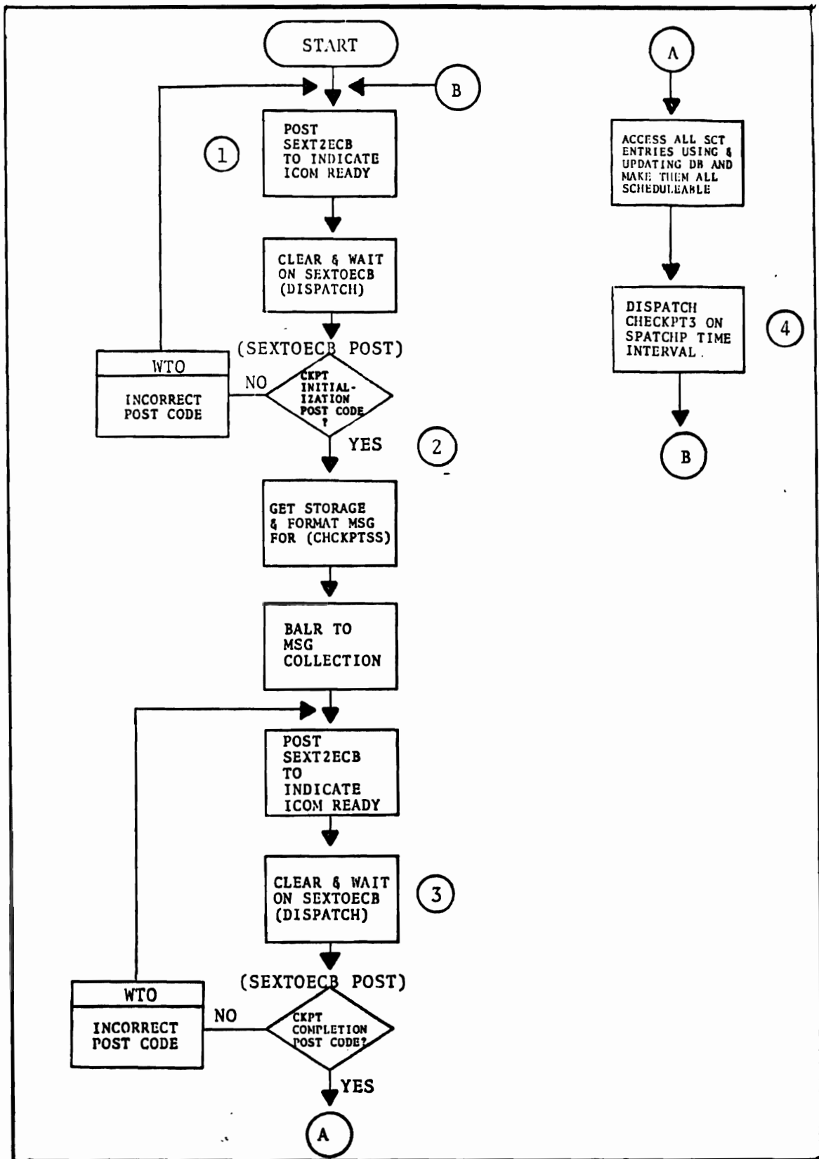
Figure 5-6. GDBSTUP Logic. (Encircled numbers correspond to list on previous page).
