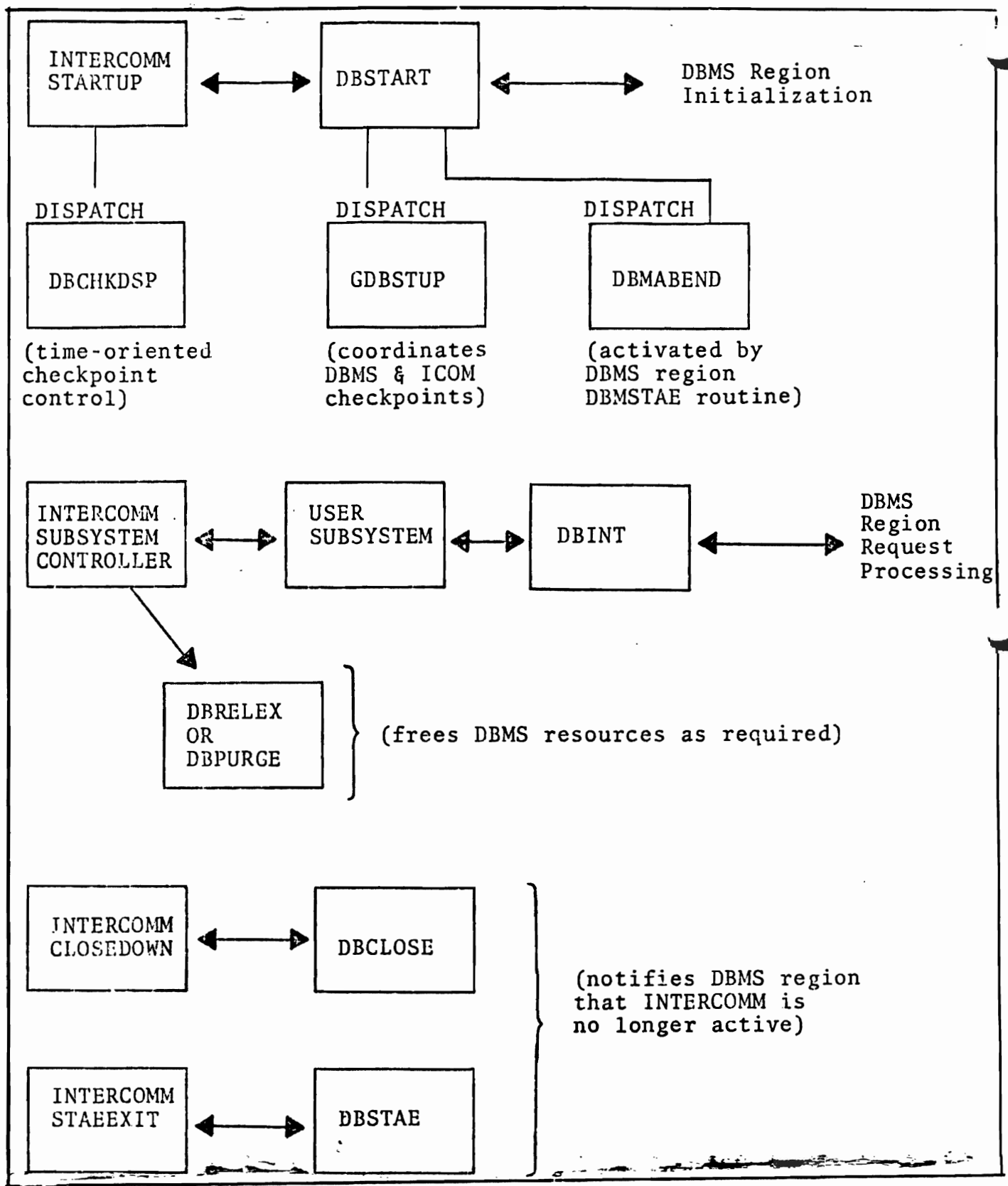
Figure 2-1. DBMS Interface Routine Summary
