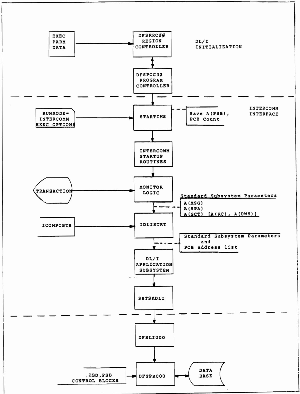
Figure 6-2. INTERCOMM-DL/I Interface Overview
