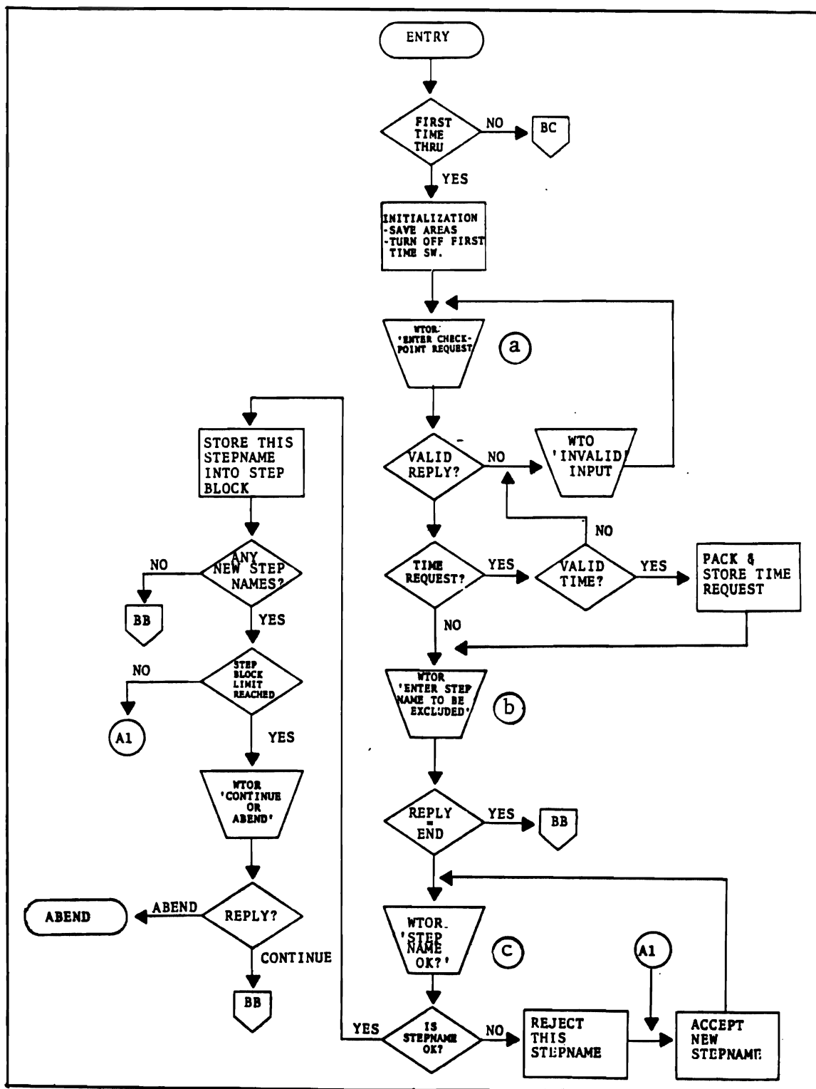
Figure 5-8. Data Base Backout First Time (Initialization)
