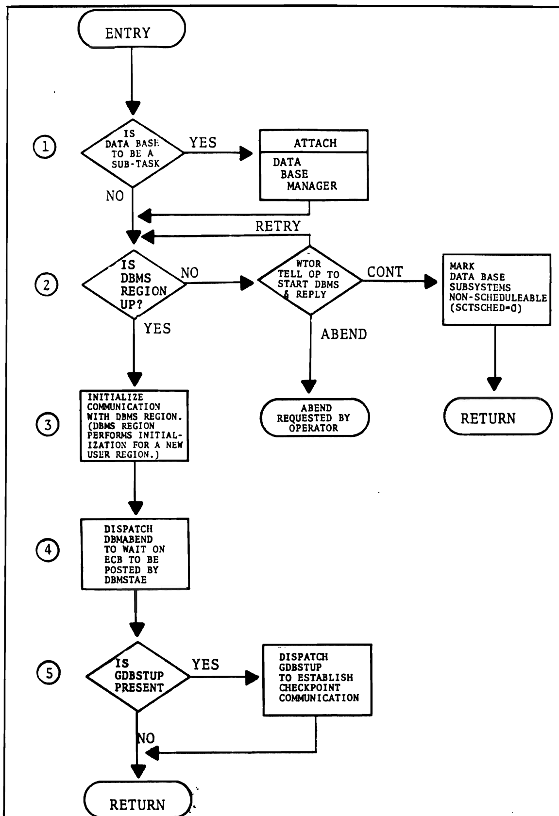
Figure 5-5. Suggested DBSTART Logic. (Encircled numbers correspond to list on previous page).
