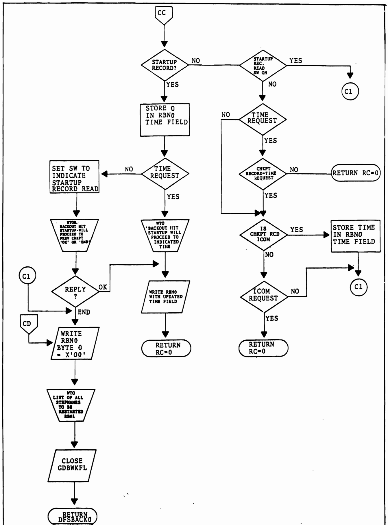
Figure 5-10. Data Base Backout Checkpoint Analysis
