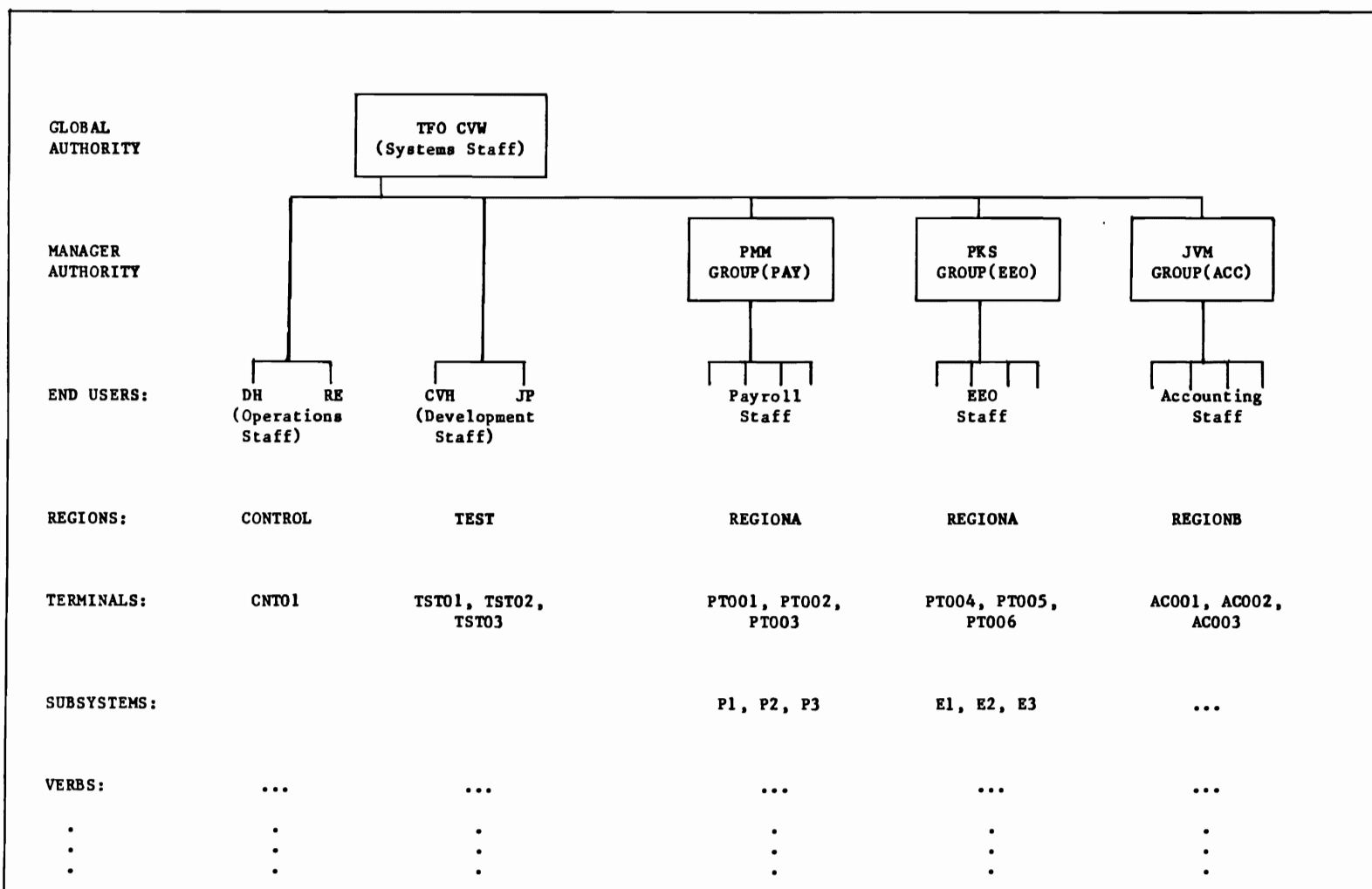
Figure 3. Security Tree
