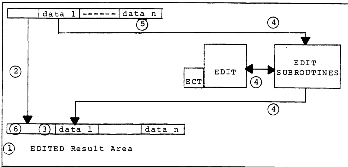
Figure 3. EDIT Control Routine Logic
